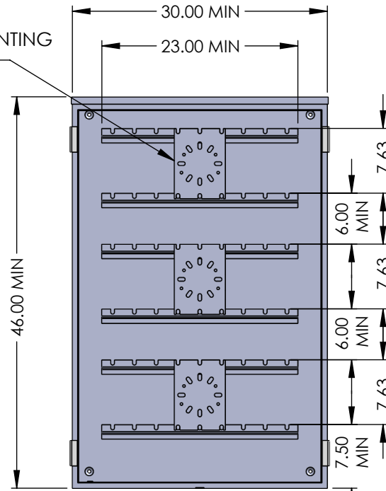
OPENED VIEW
